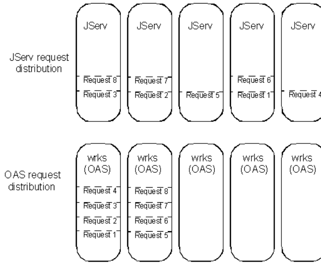
Figure 3–1 Request distribution
